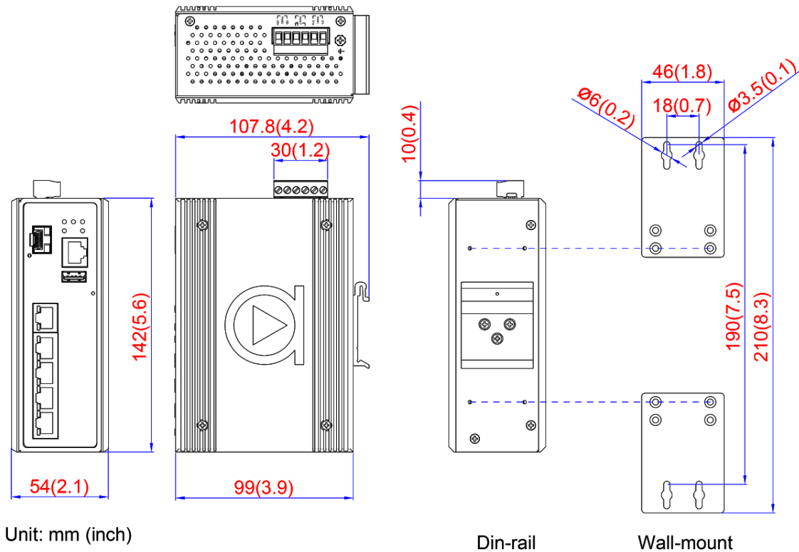
Figure 2.1 - Physical Dimensions
